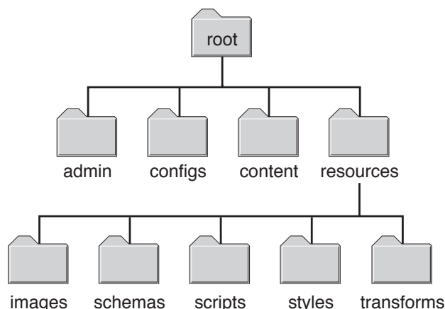
Figure 10.1: Authentication Directory
