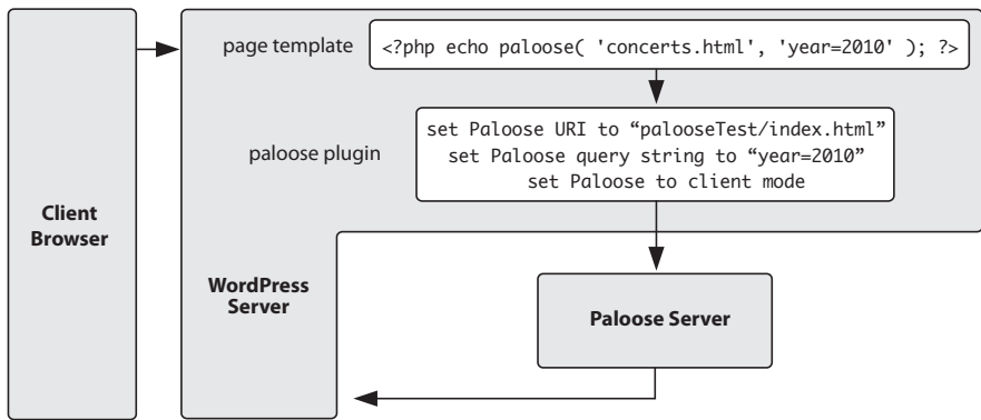
Figure 1.2: Paloose Client
