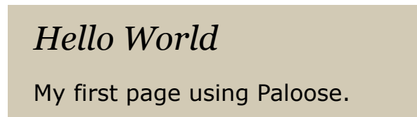
Figure 3.1: First Site
