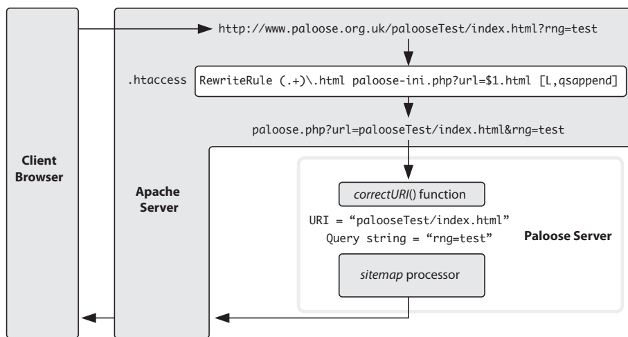
Figure 1.1: Server Client
