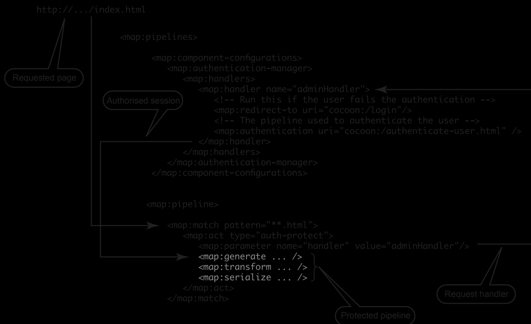
Figure 10.2: Administration Flow
