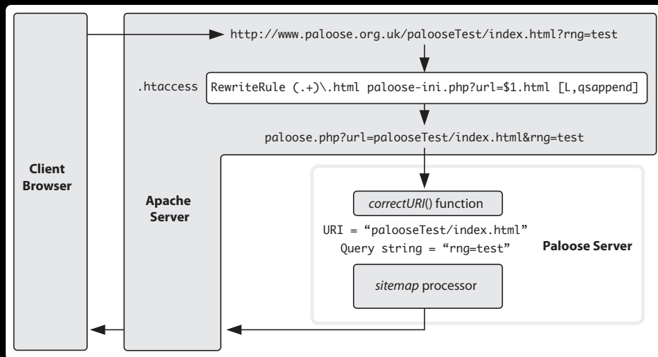
Figure 1.1: Server Client
