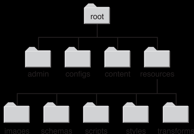
Figure 10.1: Authentication Directory
