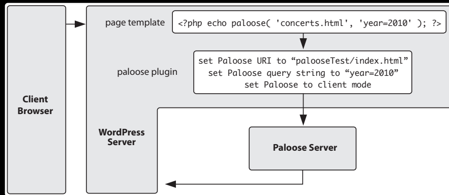
Figure 1.2: Paloose Client
