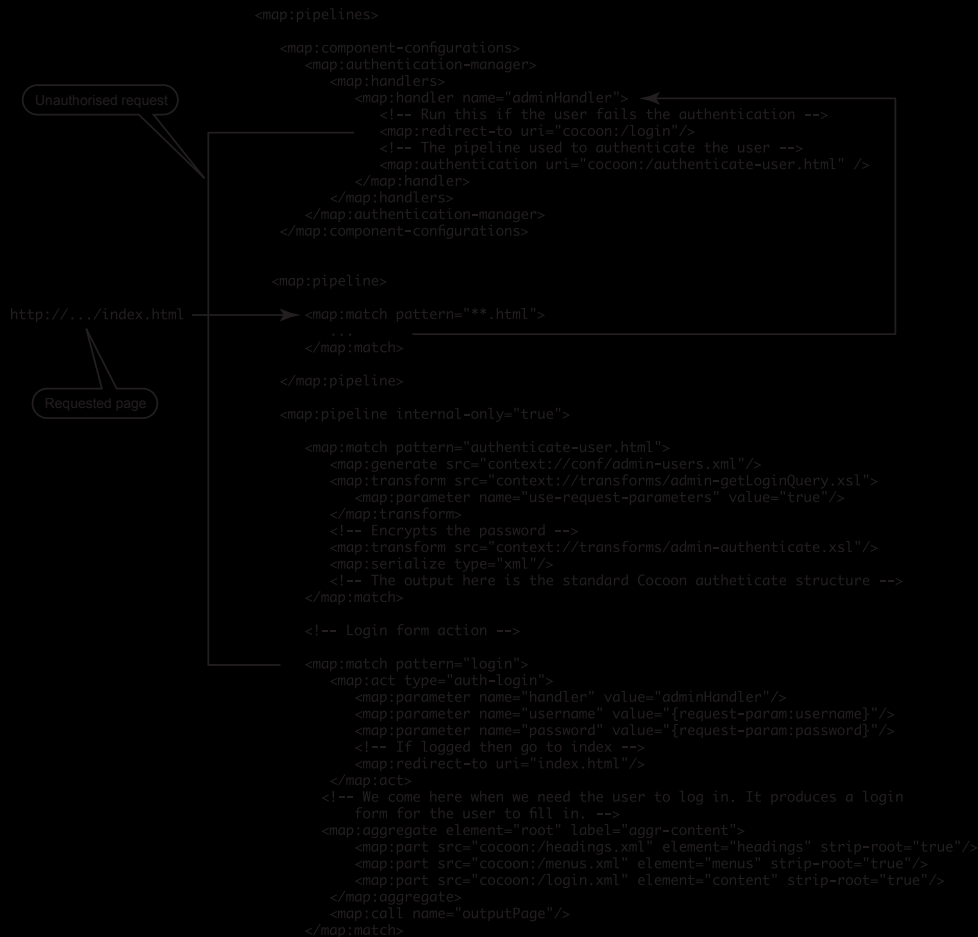
Figure 10.3: Login Flow
